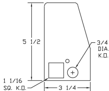
LEFT END PLATE w/ KOs
