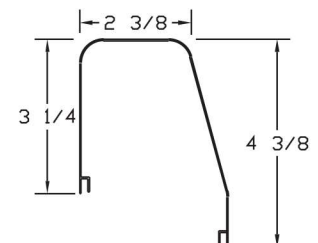
DIFFUSER
