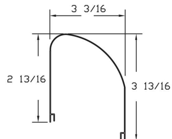
DIFFUSER
