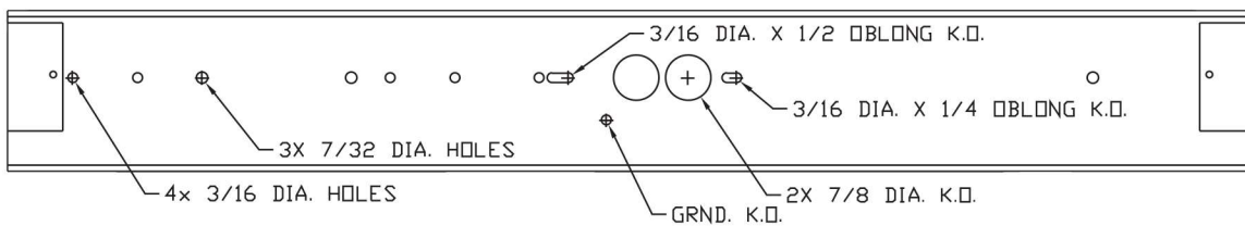
COVER (SHOWN W/ LED)
