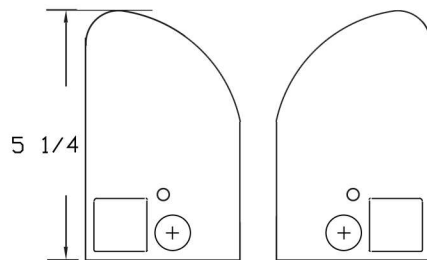
LEFT END PLATE
