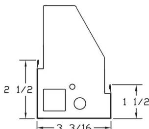
END W/O PLATE
